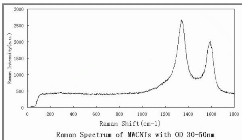
Raman Spectra
